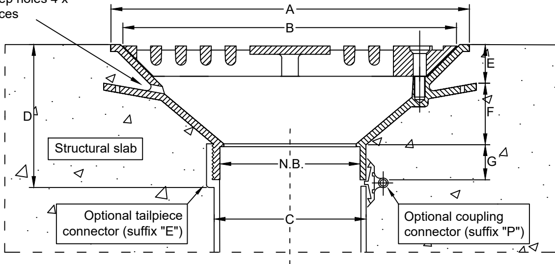
Dimensions (mm)
