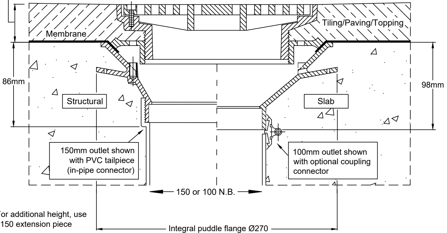
Typical Application
