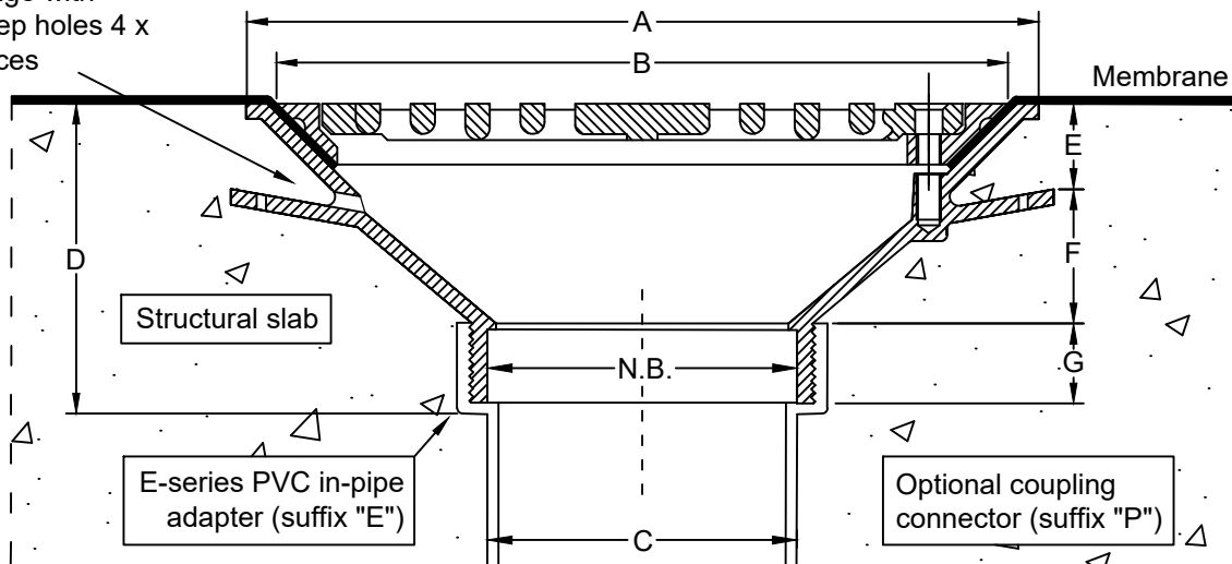
Dimensions (mm)
